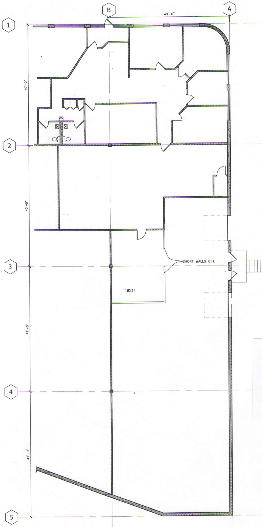
1 FLOOR PLAN- 15151 A 1/8"=1'-0"
